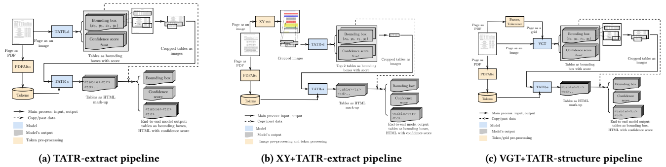
Figure 8: Pipeline for table extraction
