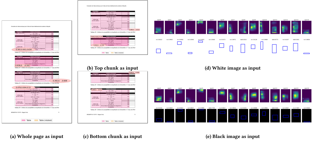
Figure 9: Left part (9a, 9b, 9c) shows how TATR’s confidence scores change. Confidence scores are ordered following the class “table”, “rotated table” and “no object”. If the dominant class is “tables” , the distribution is surrounded by a frame, otherwise (“no object” dominant) it is an ellipse. Right part (9d, 9e) shows query location.
