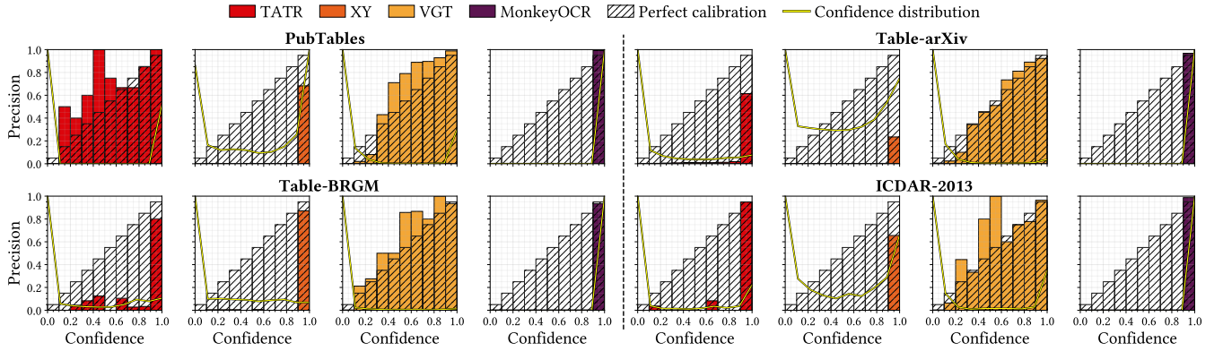
Figure 12: Reliability diagrams of probabilistic models across datasets
