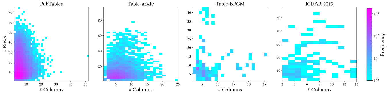
Figure 7: Distribution of the numbers of rows and columns in our datasets
