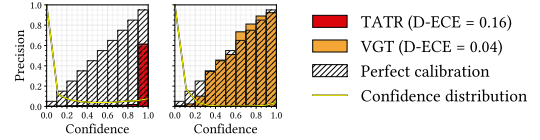
Figure 4: Reliability diagrams on Table-arXiv.
