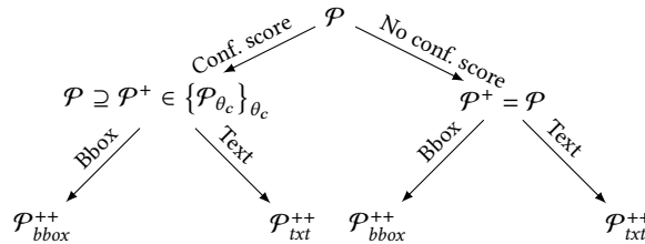
Figure 10: TSR inputs depending on the TD model type (with or without a confidence score), and evaluation type ( bbox -based or txt -based).
