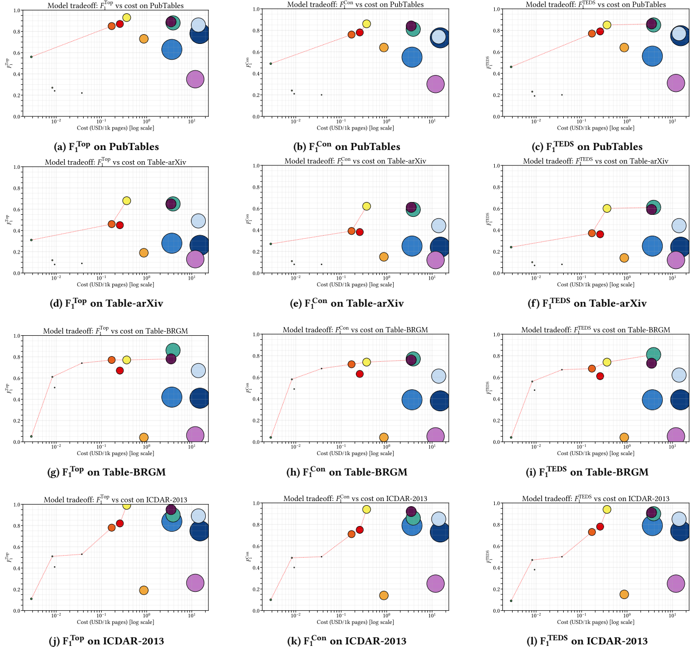
Figure 16: Tradeoff: TE metrics vs. computational cost for each txt TE metric across datasets. Bubble size is roughly proportional to the logarithm number of parameters (see Figure 1). Colors are the same as in Figure 1 and Table 2.
