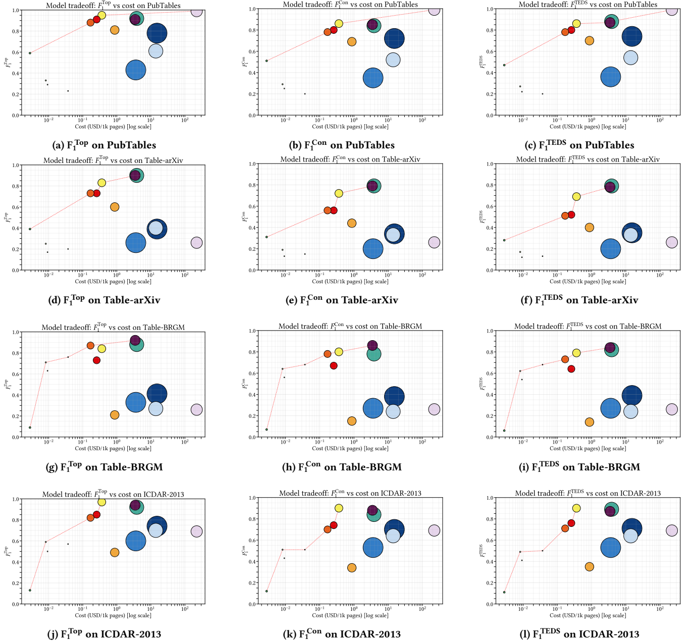
Figure 15: Tradeoff: TE metrics vs. computational cost for each bbox TE metric across datasets. Bubble size is roughly proportional to the logarithm number of parameters (see Figure 1). Colors are the same as in Figure 1 and Table 2.
