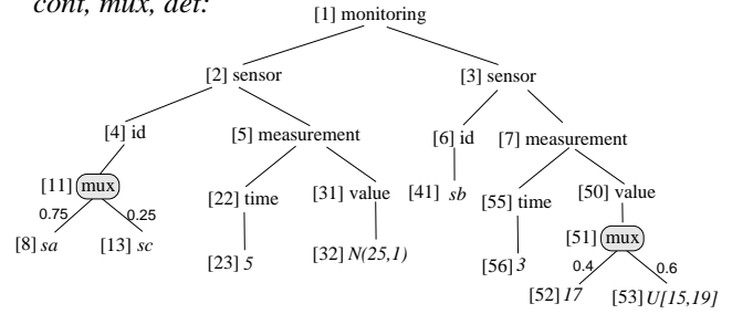
Figure 6: \text{PrXML}^{\text{cont, mux, det}} p-document: monitoring.
