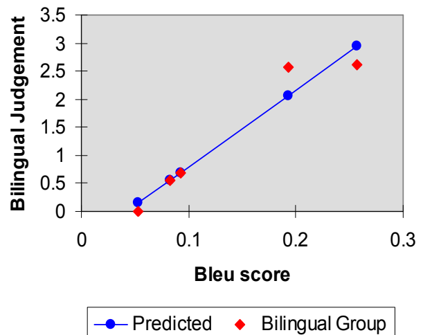
Figure 6: BLEU predicts Bilingual Judgments
