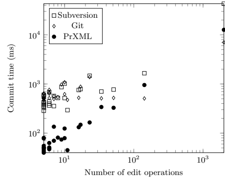
Figure 5: Commit time vs number of edit operations (for edit scripts of length \geq 5 )
