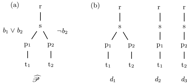
Figure 2: (a) \text{PrXML}^{\text{fie}} p-document \widehat{\mathcal{P}} ; (b) Three possible worlds d_1, d_2 and d_3
