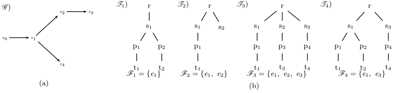
Figure 3: (a) Graph of Version Space; (b) Four versions and their corresponding truth-values
