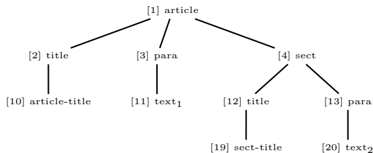
Figure 1: Example XML tree \mathcal{T} : Wikipedia article
